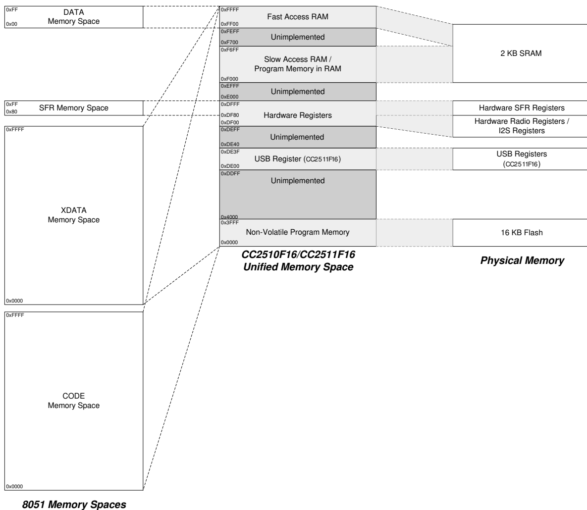
Figure 15: CC2510F16/CC2511F16 Memory Mapping
